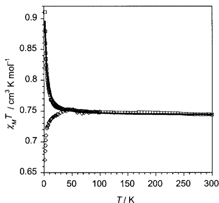
Figure 3. Experimental \chi_M T versus T behavior for compounds 5a (tilted squares) and 5b (squares); the solid line represents the calculated best fit to the experimental data for 5b .
