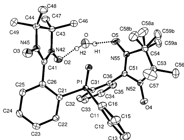
Figure 2. ORTEP drawing for compound 5b (30% probability ellipsoids); selected bond lengths and distances [Å] and angles [°]: O2–N42 1.288(2), O3–N45 1.278(2), O4–N52 1.283(2), O5–N55 1.280(2), C41–N42 1.334(2), C41–N45 1.351(3), C26–C41 1.476(3), C21–C26 1.409(3), C51–N52 1.341(2), C51–N55 1.341(3), C36–C51 1.477(3), P–O1 1.480(2), P–C11 1.811(2), P–C21 1.821(2), P–C31 1.827(2) O2...H2 2.03(3), O5...H1, 1.94(3); O2–O–O5 94.35(7), O1–P–C11 110.74(8), O1–P–C21 113.96(8), O1–P–C31 114.79(9); mean plane angles: radical–phenyl 51.56(7) and 87.26(7), radical–radical 77.09(8)
