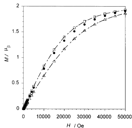
Figure 4. Experimental (black dots) field dependence of the magnetization for compound 5b at 2 K compared to the magnetization given by the Brillouin function for one S = 1 spin (squares) and two uncorrelated S = 1/2 spins (triangles) for the same temperature (the lines are just eye guides).
