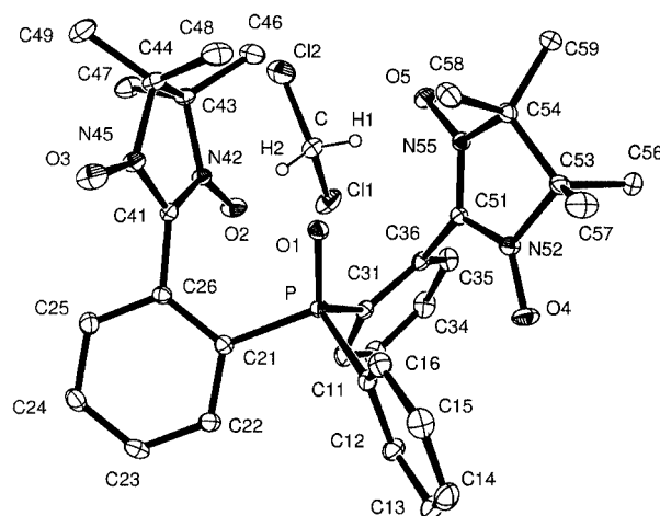
Figure 1. ORTEP drawing for compound 5a (30% probability ellipsoids); selected bond lengths [Å] and angles [°]: O2–N42 1.287(2), O3–N45 1.281(2), O4–N52 1.275(2), O5–N55 1.283(2), C41–N42 1.343(2), C41–N45 1.338(2), C26–C41 1.473(2), C21–C26 1.408(2), P–O1 1.486(1), P–C11 1.810(2), P–C21 1.825(2), P–C31 1.822(1); O1–P–C11 112.41(7), O1–P–C21 111.75(7), O1–P–C31 112.88(7); mean plane angles: radical–phenyl 68.22(5) and 78.99(5), radical–radical 67.28(6)
